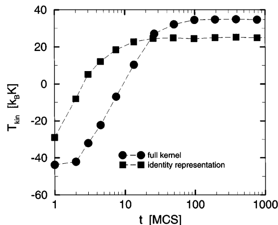
FIG. 2. Kinetic energy estimator T_{\text{kin}} as a function of time in Monte Carlo sweeps for solid \text{CH}_4 at T = 16 K with Trotter number P = 4 .
